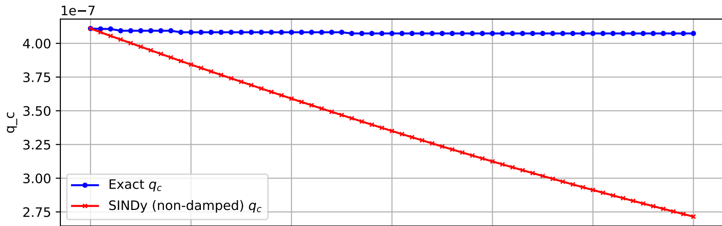
Trajectory 176 (non-damped)
