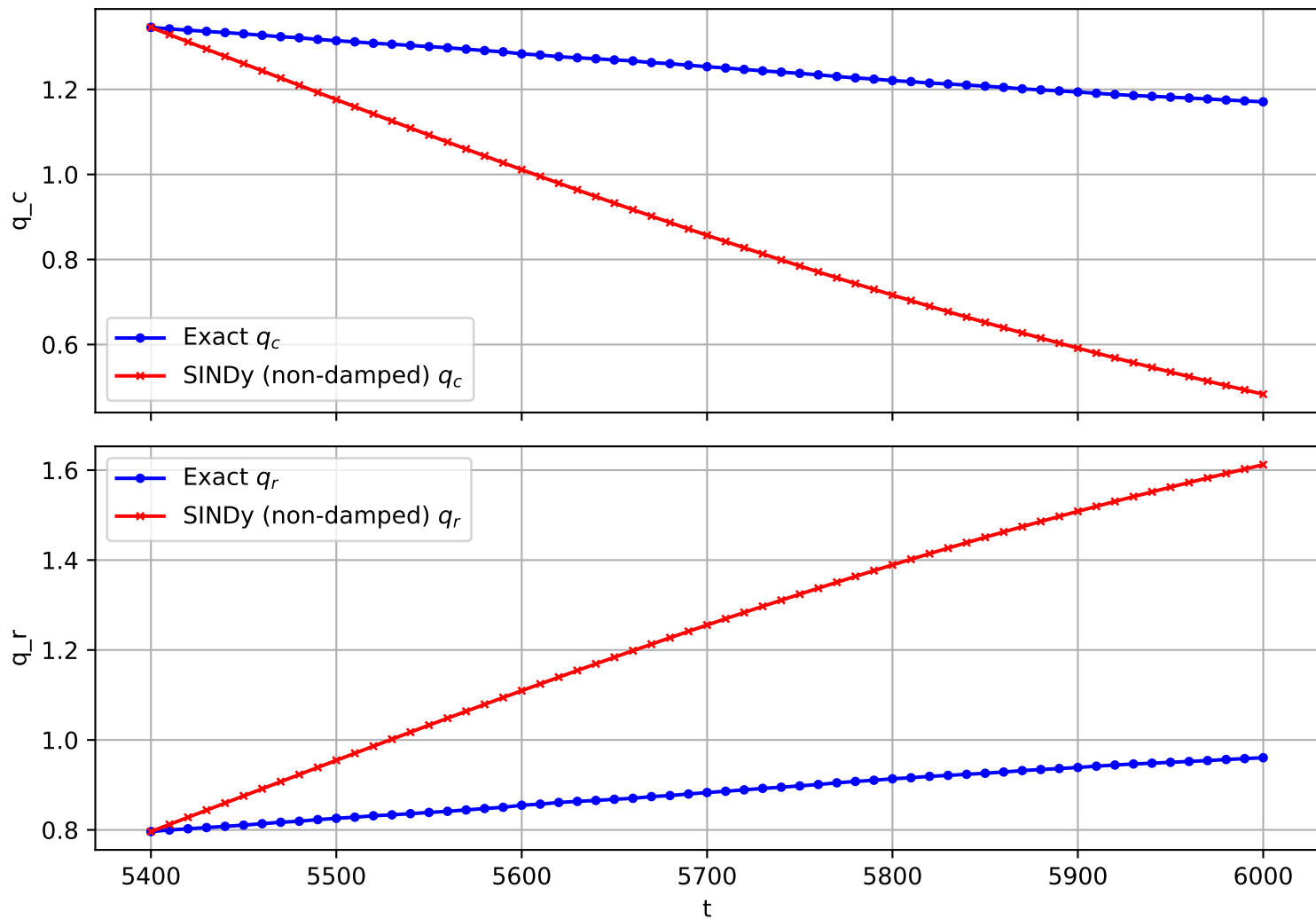
Trajectory 183 (non-damped)
