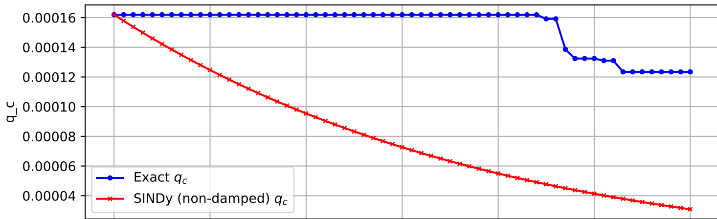
Trajectory 212 (non-damped)
