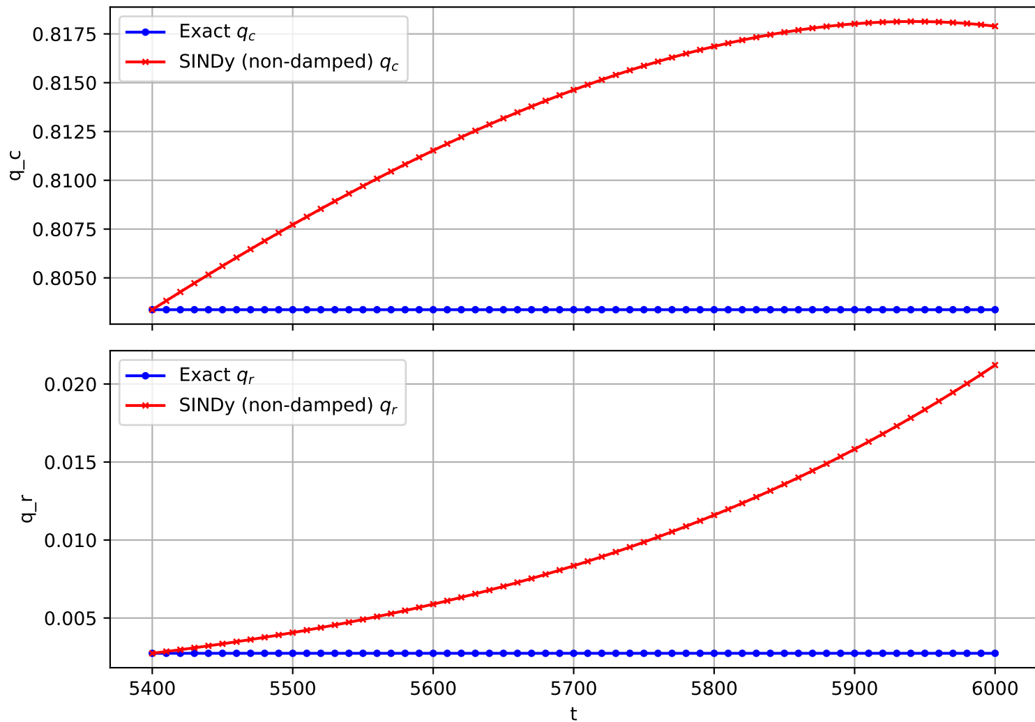
Trajectory 216 (non-damped)
