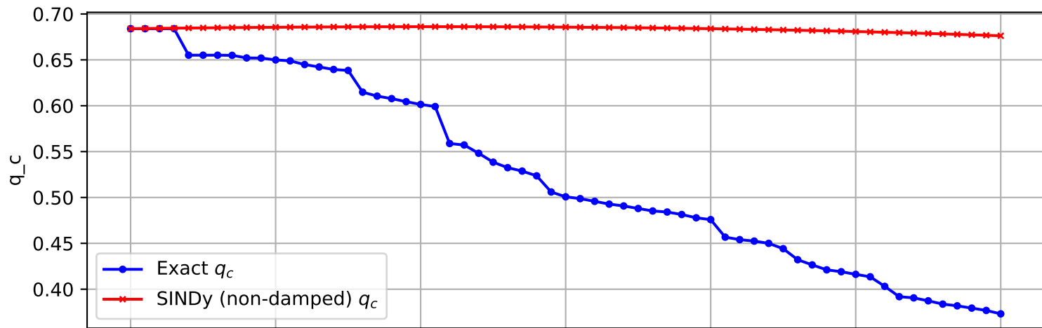
Trajectory 22 (non-damped)
