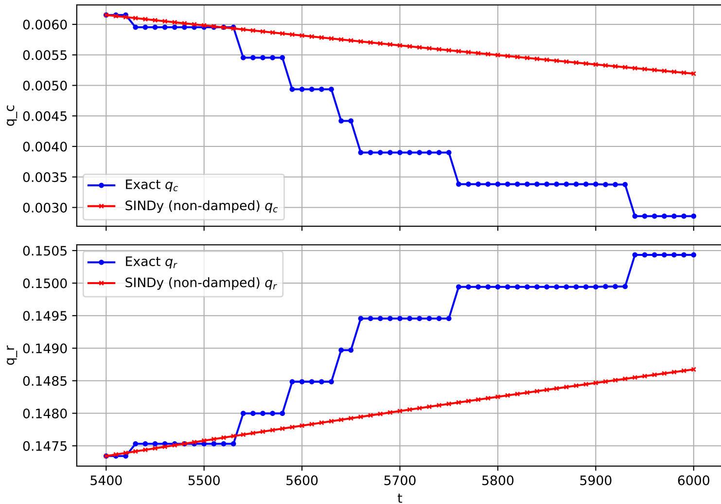
Trajectory 220 (non-damped)
