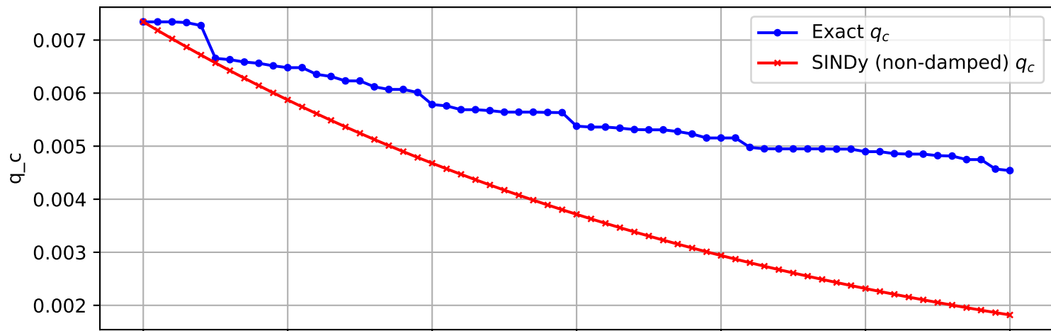
Trajectory 224 (non-damped)
