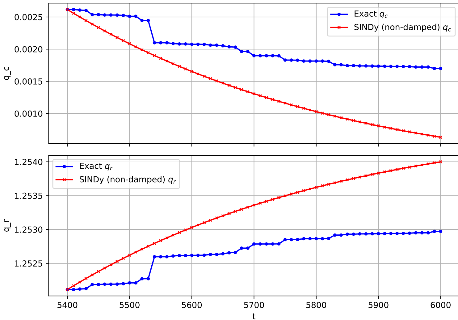
Trajectory 228 (non-damped)
