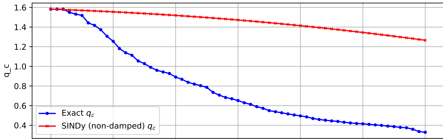
Trajectory 238 (non-damped)
