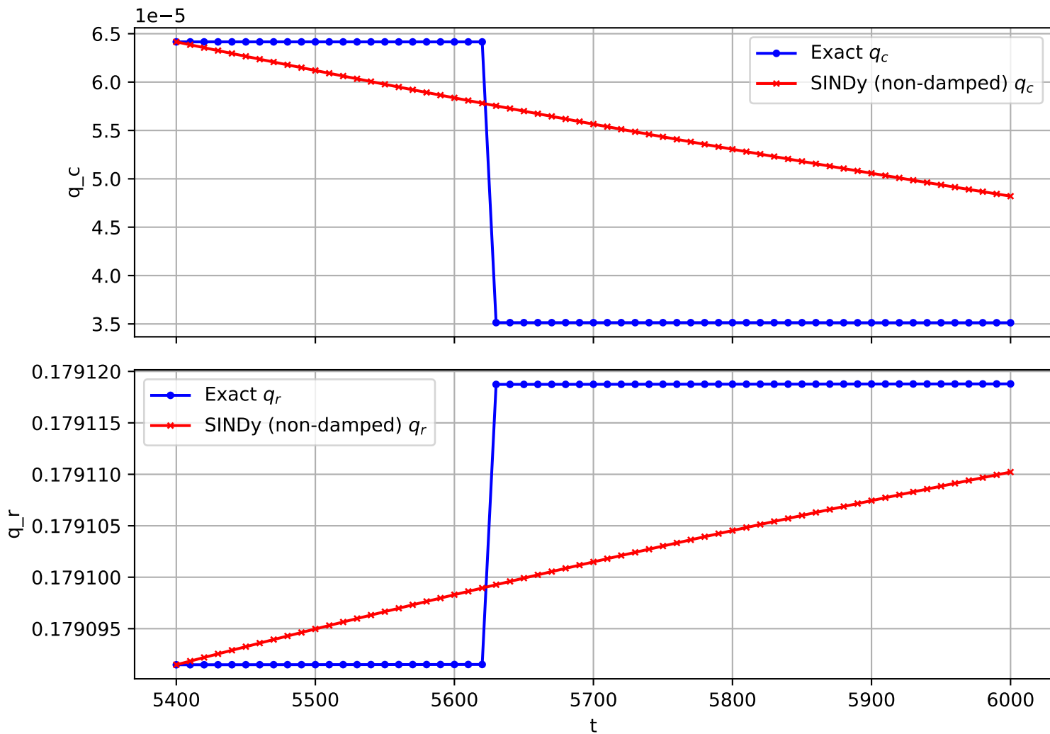
Trajectory 245 (non-damped)
