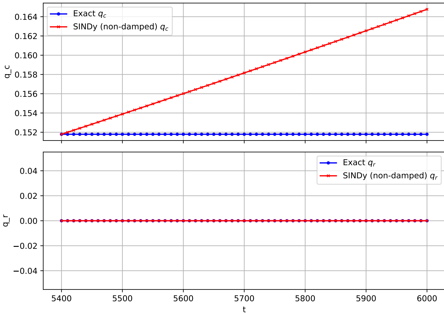
Trajectory 247 (non-damped)
