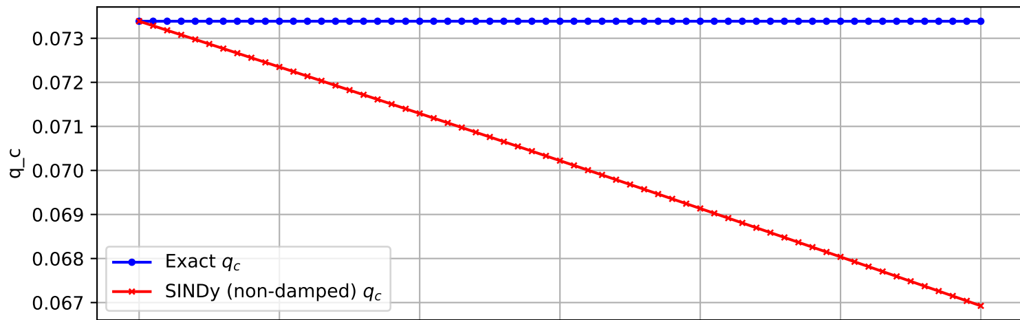
Trajectory 25 (non-damped)
