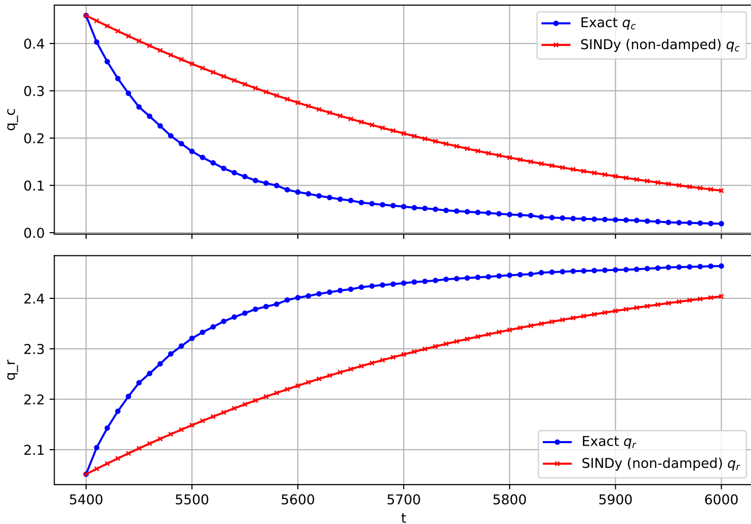
Trajectory 252 (non-damped)
