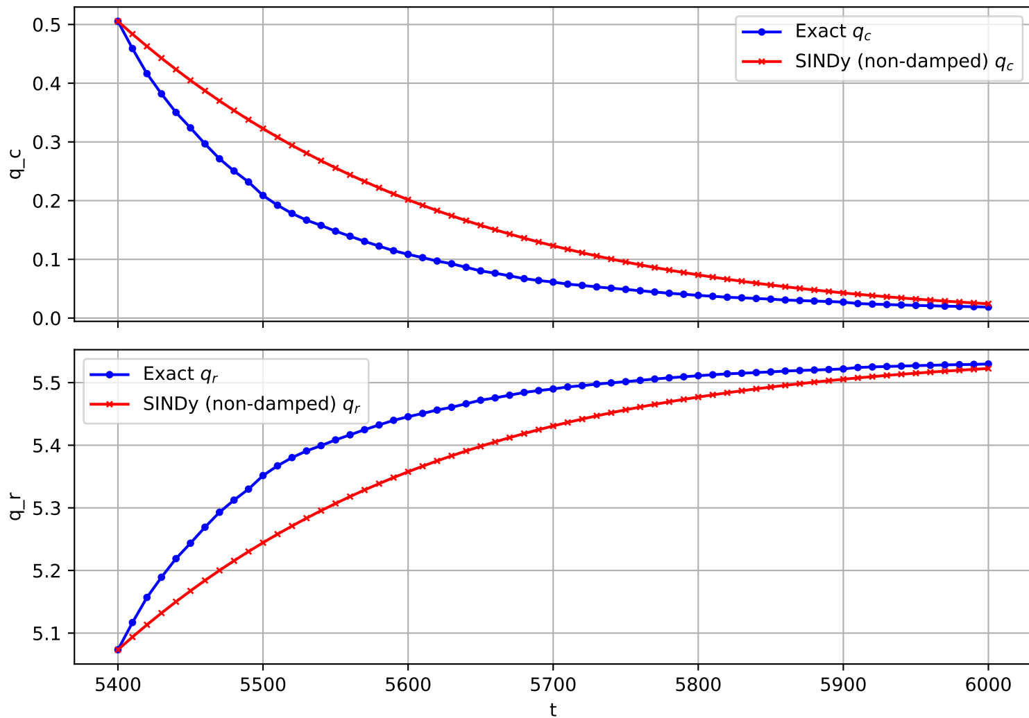
Trajectory 258 (non-damped)
