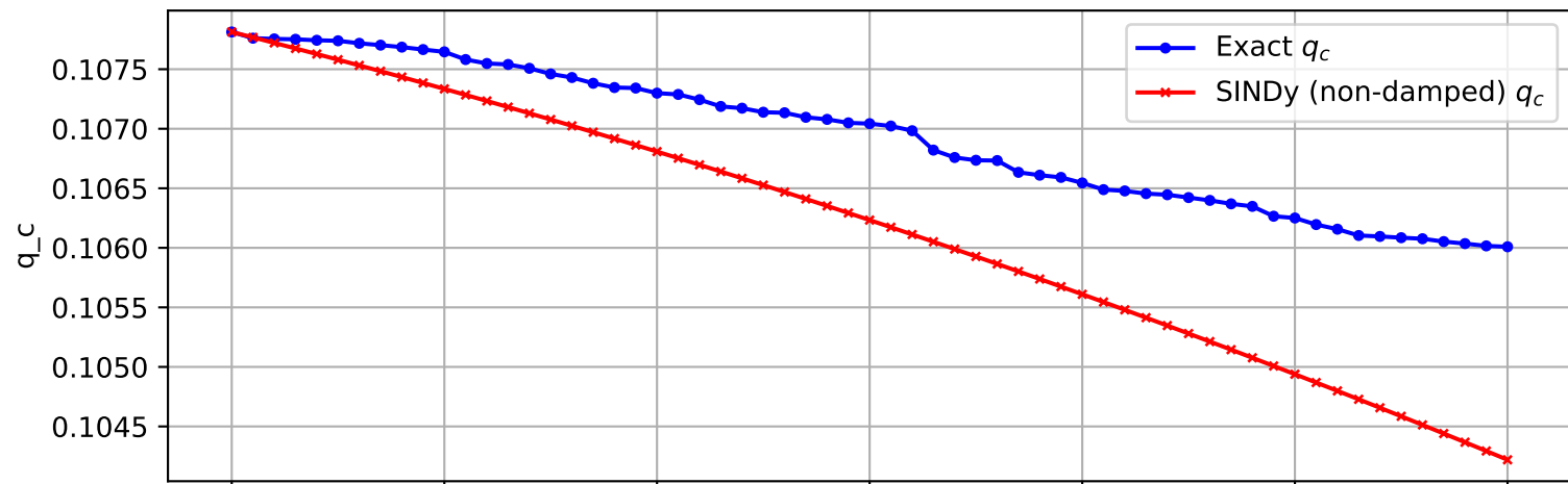
Trajectory 26 (non-damped)
