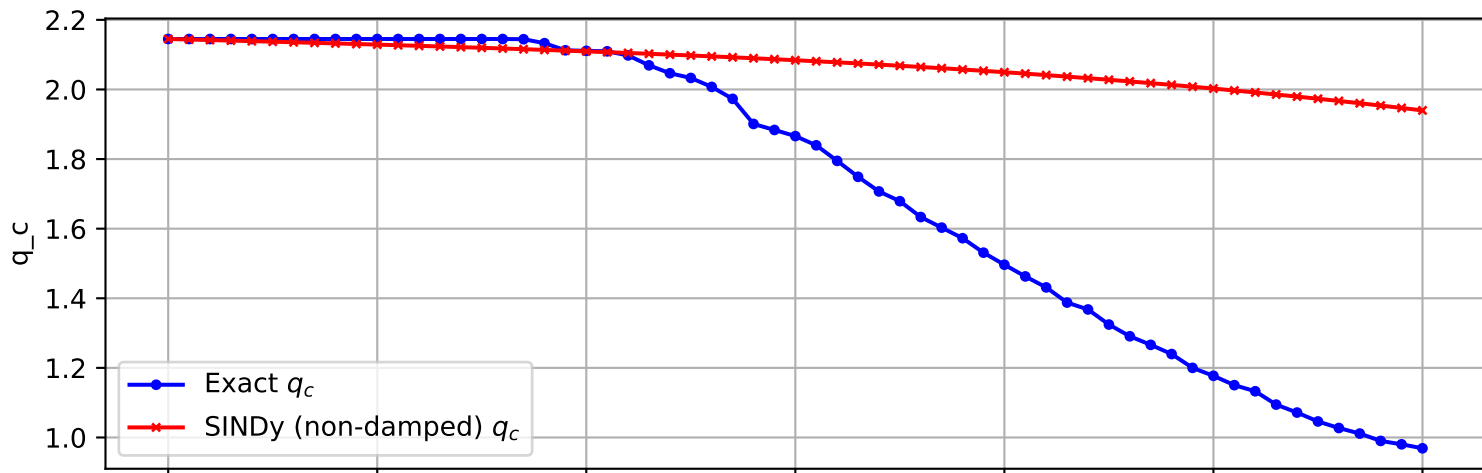
Trajectory 262 (non-damped)
