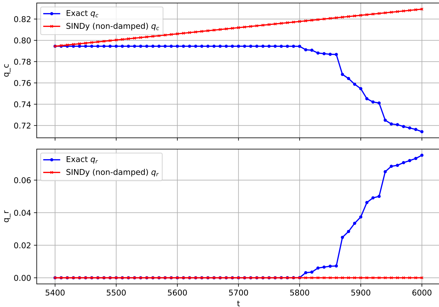
Trajectory 265 (non-damped)
