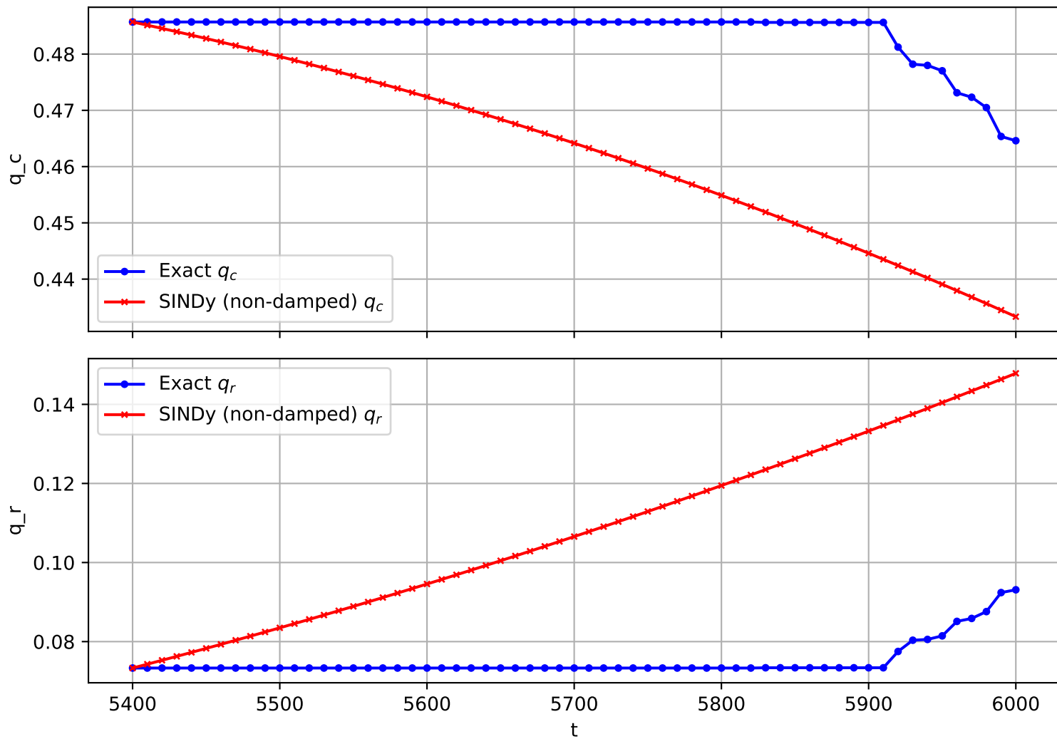
Trajectory 272 (non-damped)
