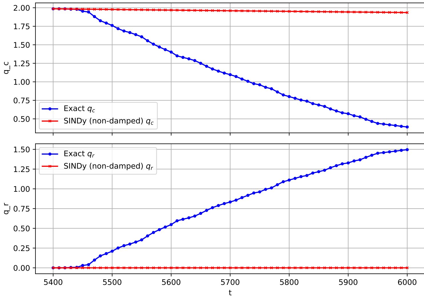
Trajectory 274 (non-damped)
