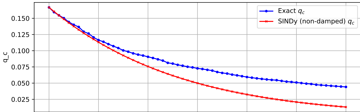
Trajectory 294 (non-damped)
