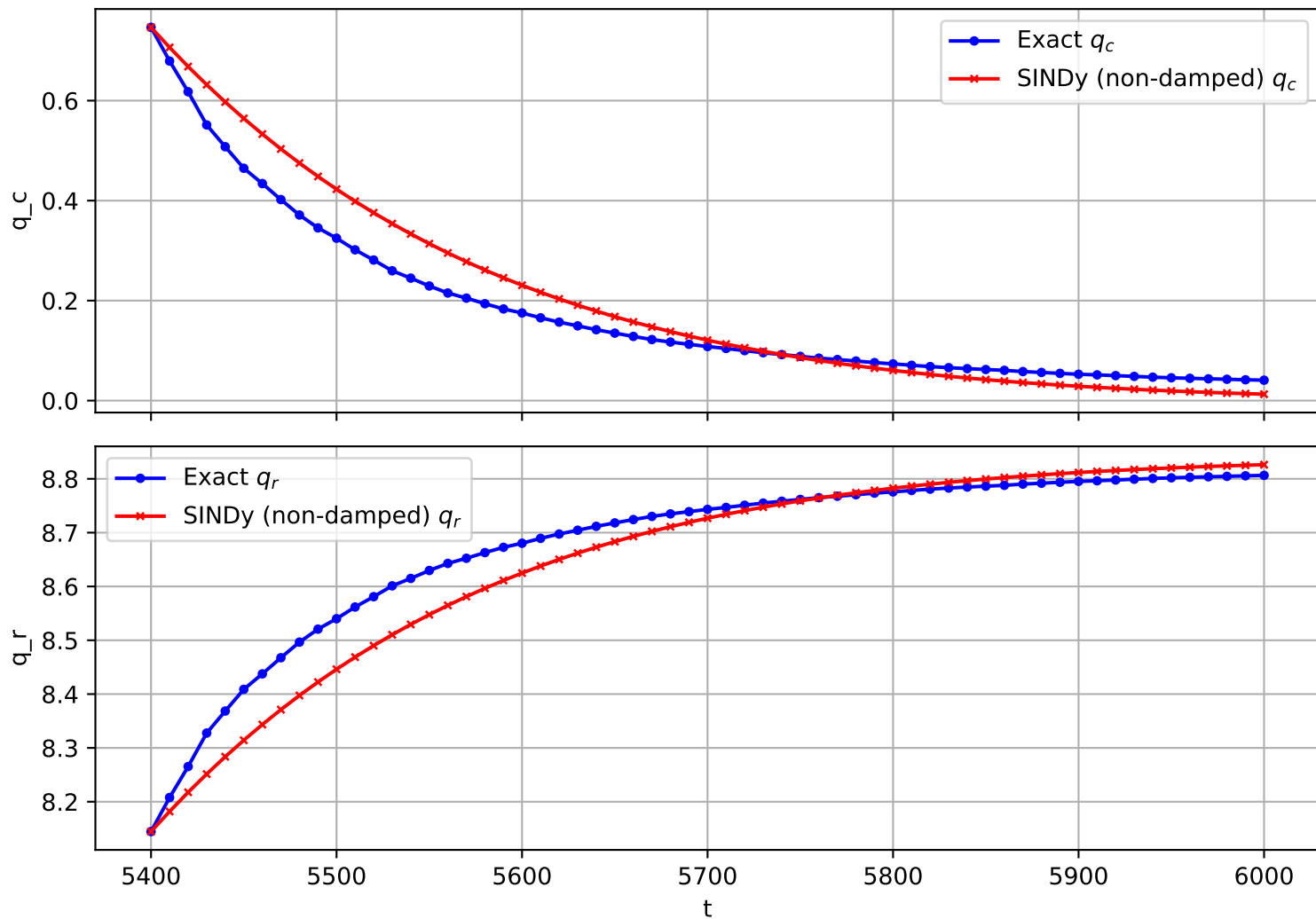
Trajectory 295 (non-damped)
