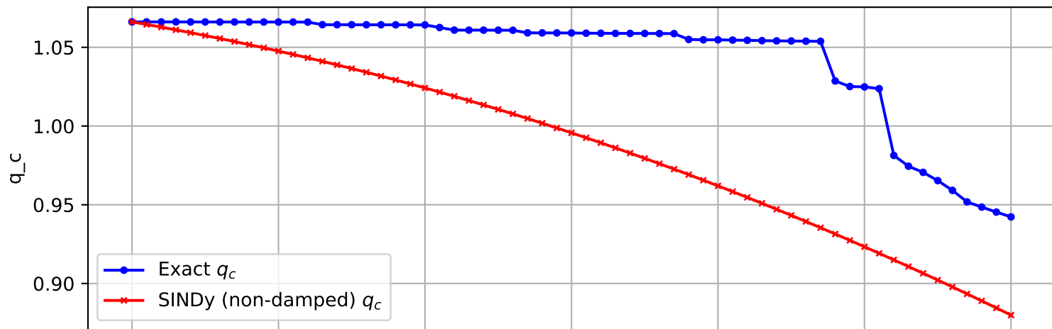
Trajectory 3 (non-damped)
