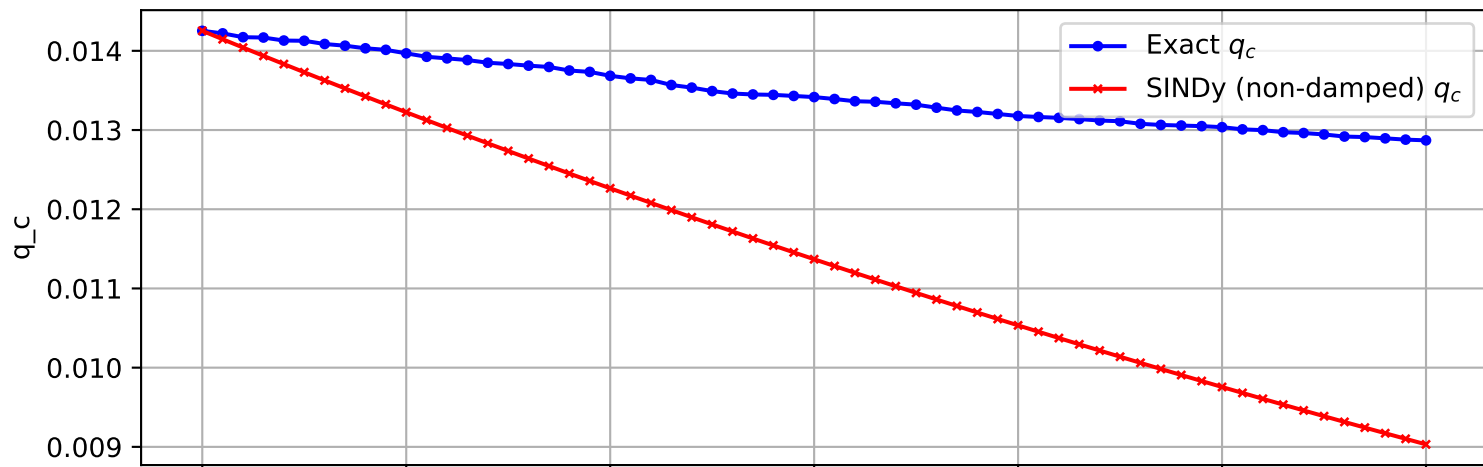
Trajectory 30 (non-damped)
