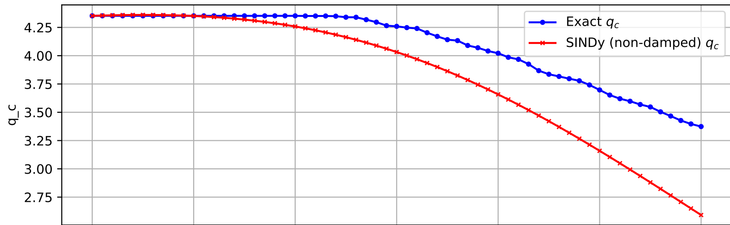
Trajectory 304 (non-damped)
