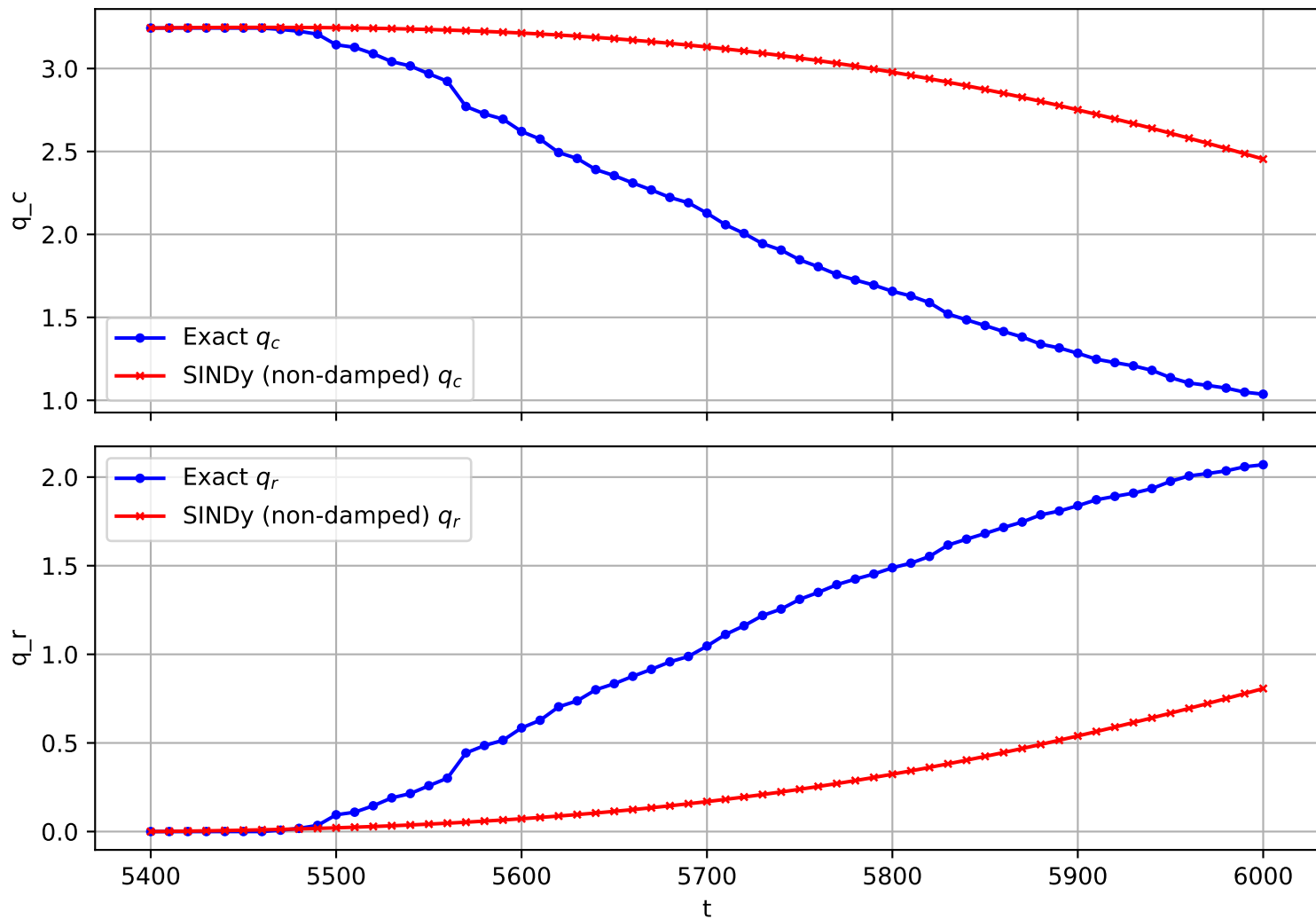
Trajectory 314 (non-damped)
