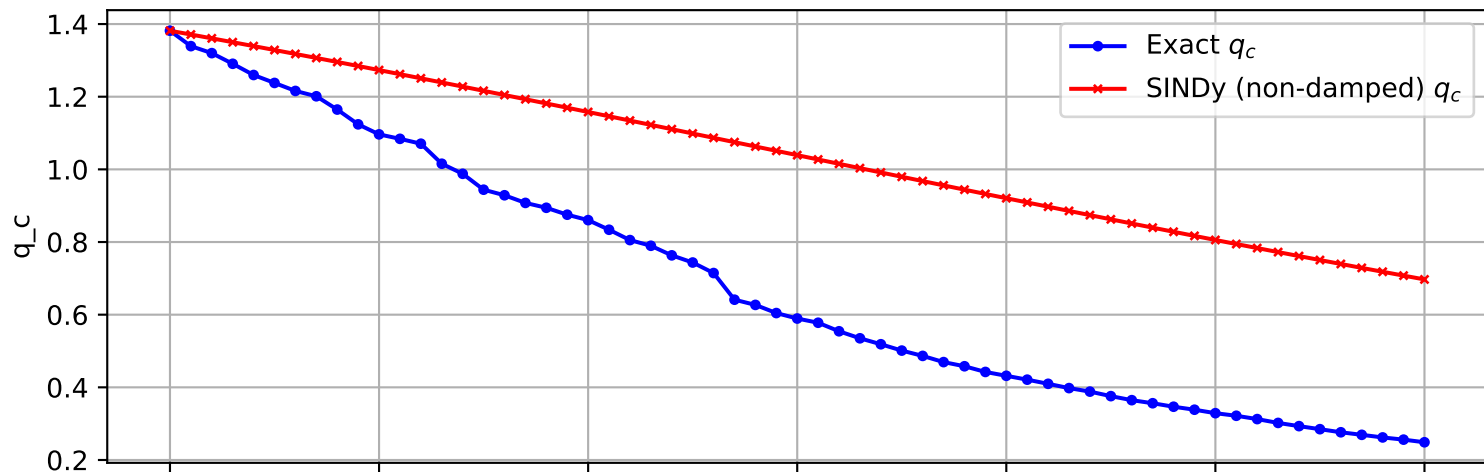
Trajectory 328 (non-damped)
