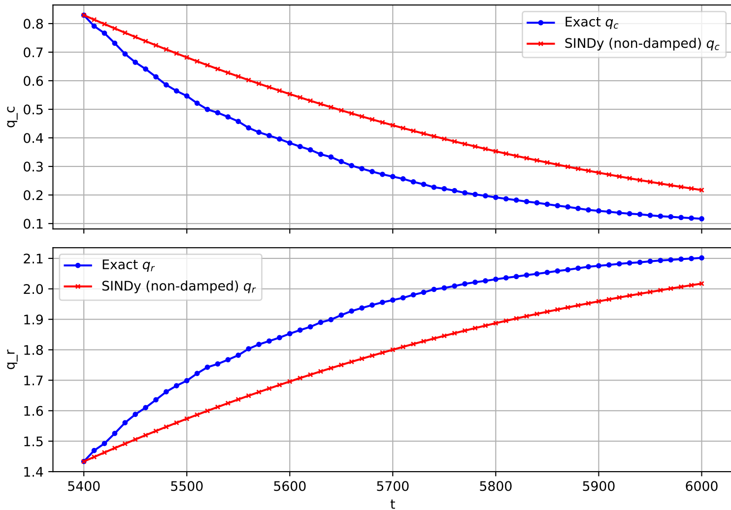
Trajectory 33 (non-damped)
