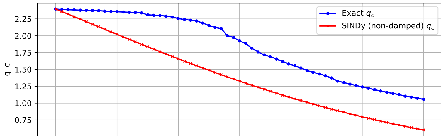
Trajectory 335 (non-damped)
