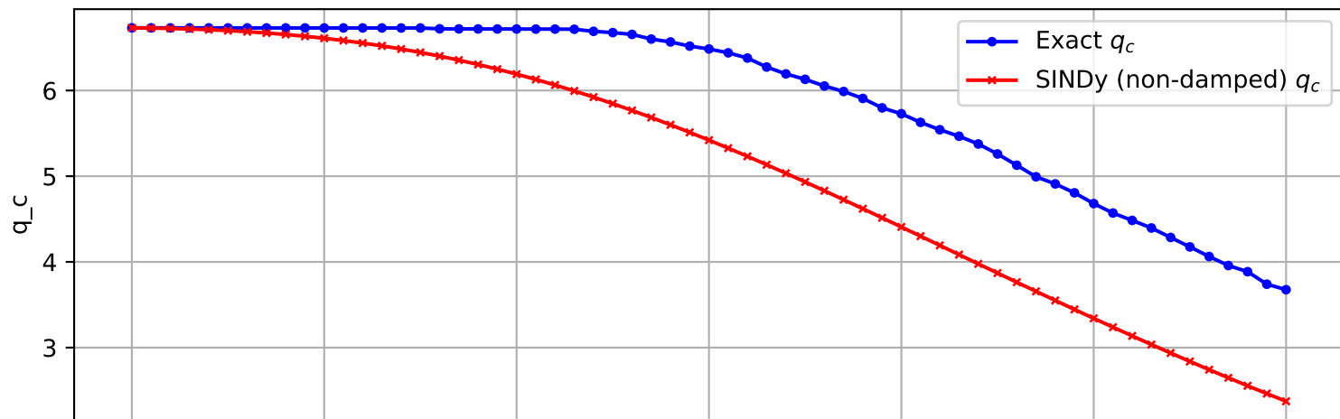
Trajectory 340 (non-damped)
