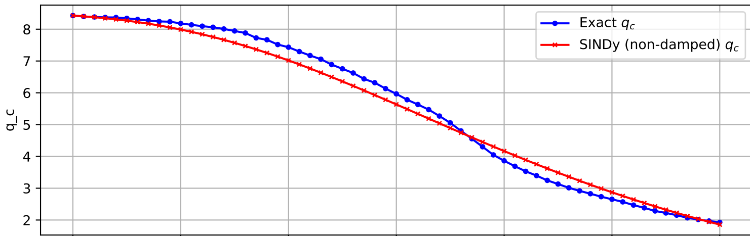
Trajectory 341 (non-damped)
