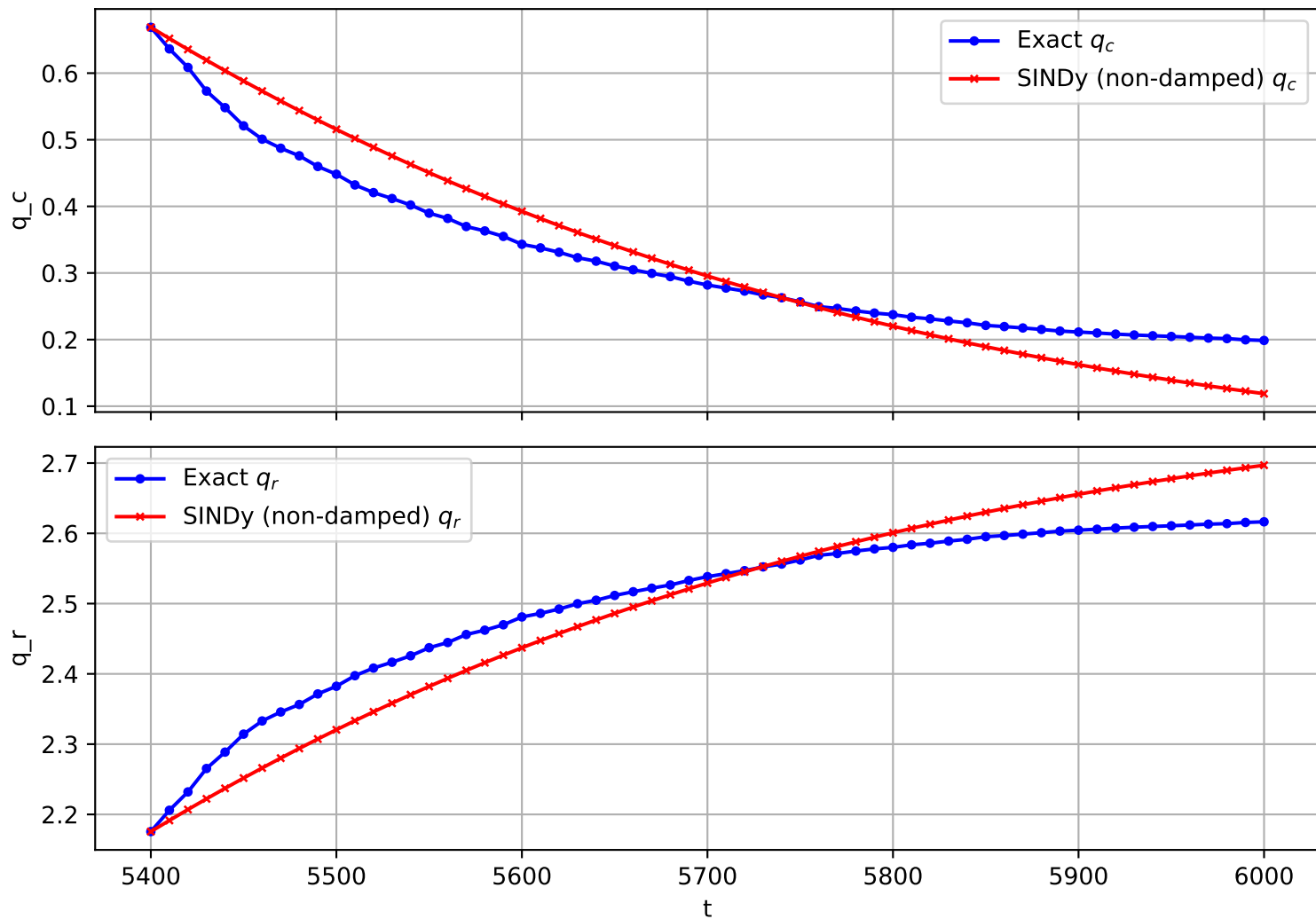
Trajectory 35 (non-damped)
