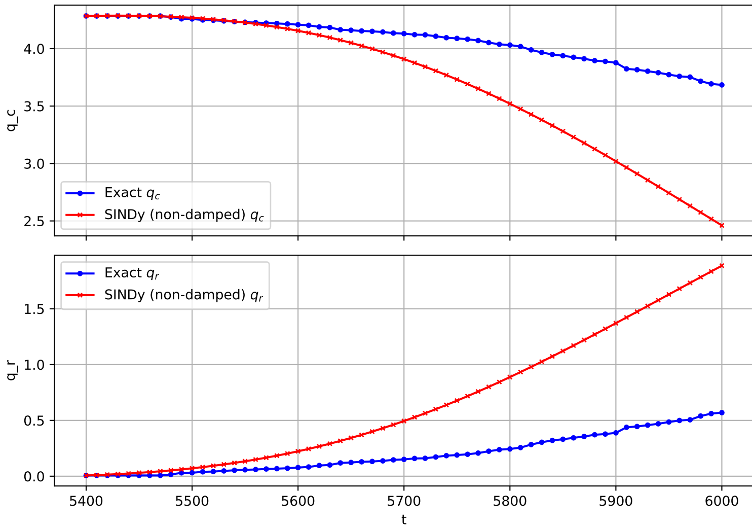
Trajectory 360 (non-damped)
