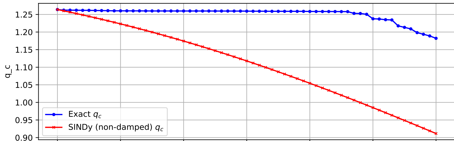
Trajectory 378 (non-damped)
