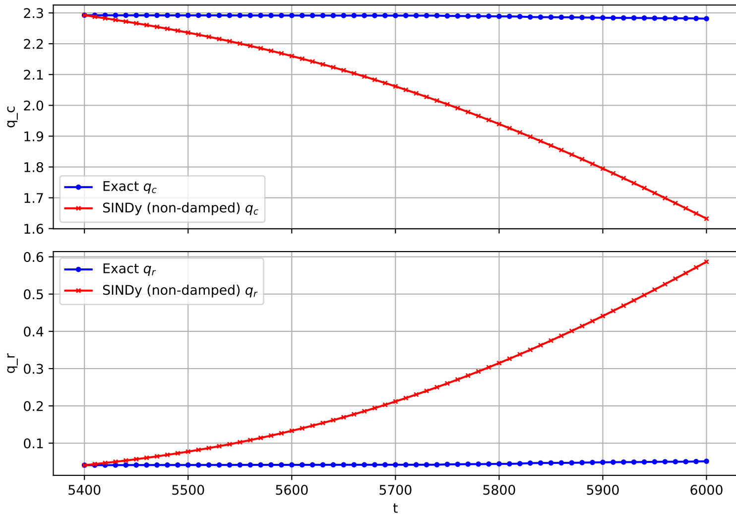
Trajectory 382 (non-damped)
