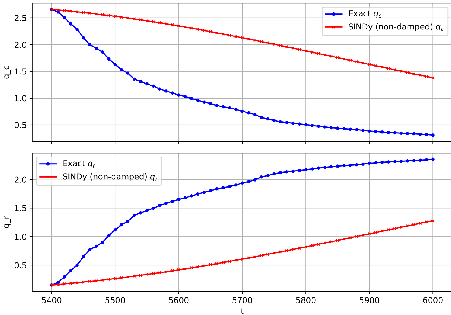
Trajectory 389 (non-damped)
