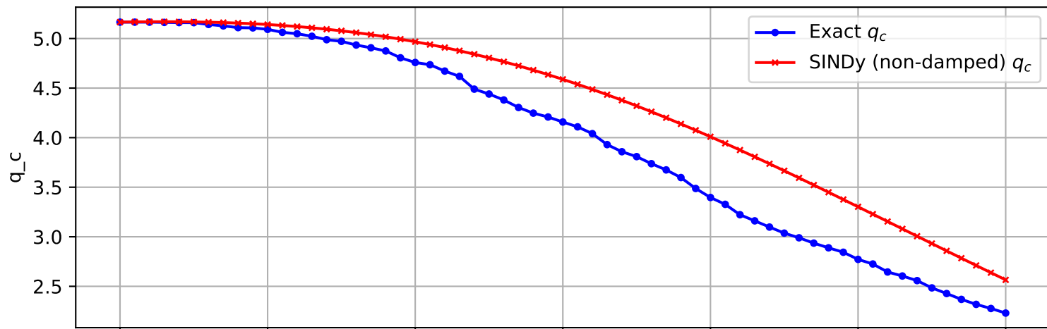
Trajectory 396 (non-damped)
