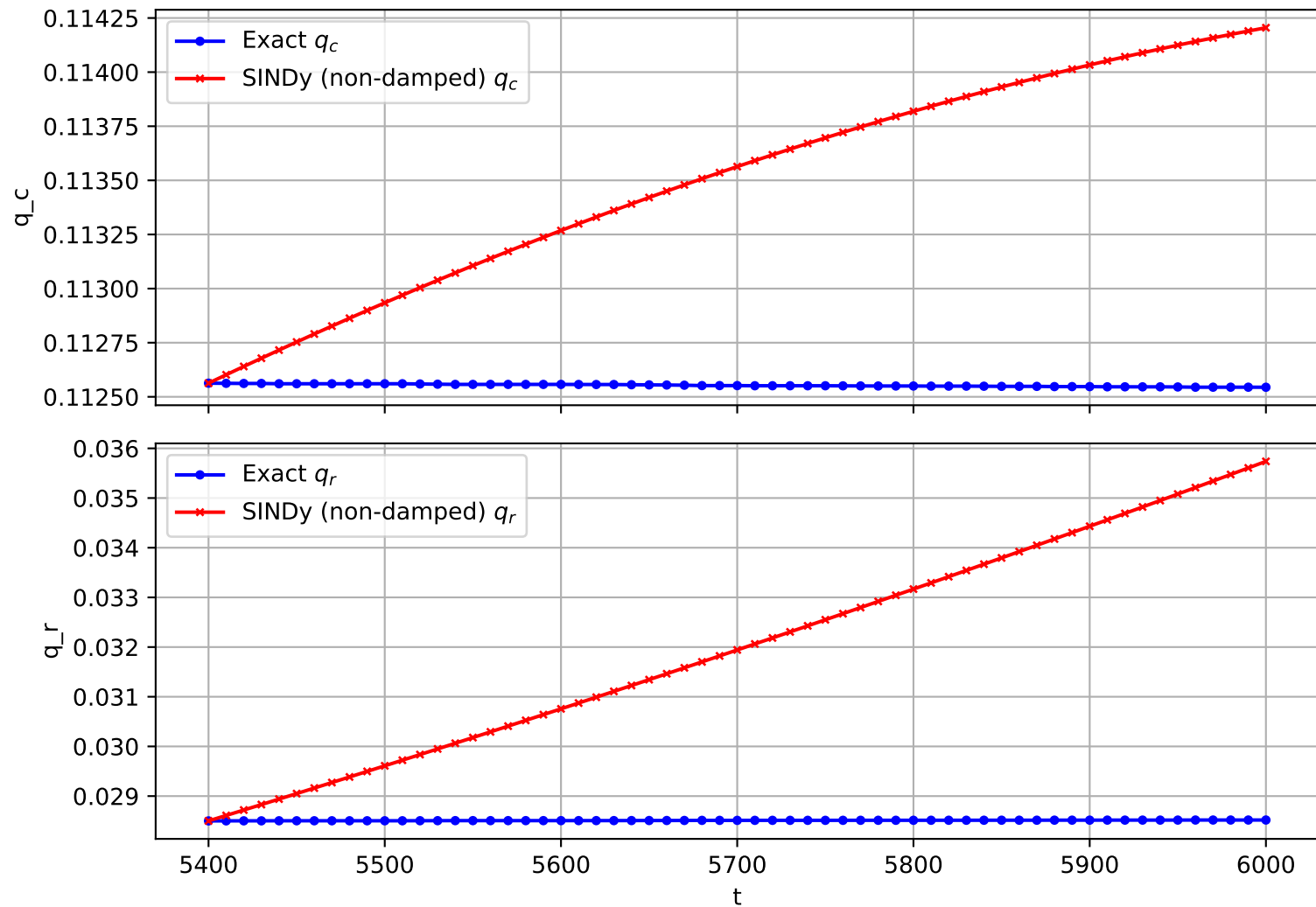
Trajectory 405 (non-damped)
