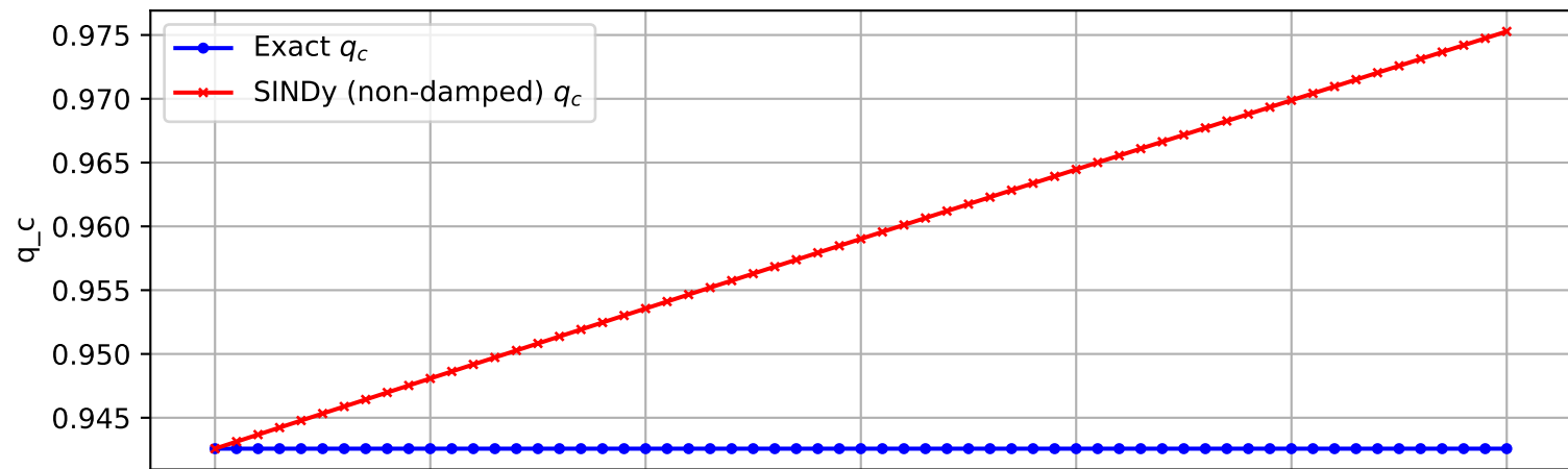
Trajectory 407 (non-damped)
