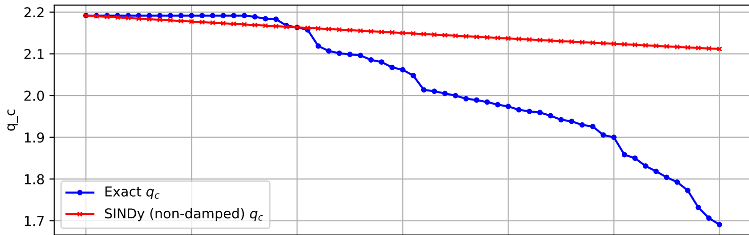
Trajectory 42 (non-damped)
