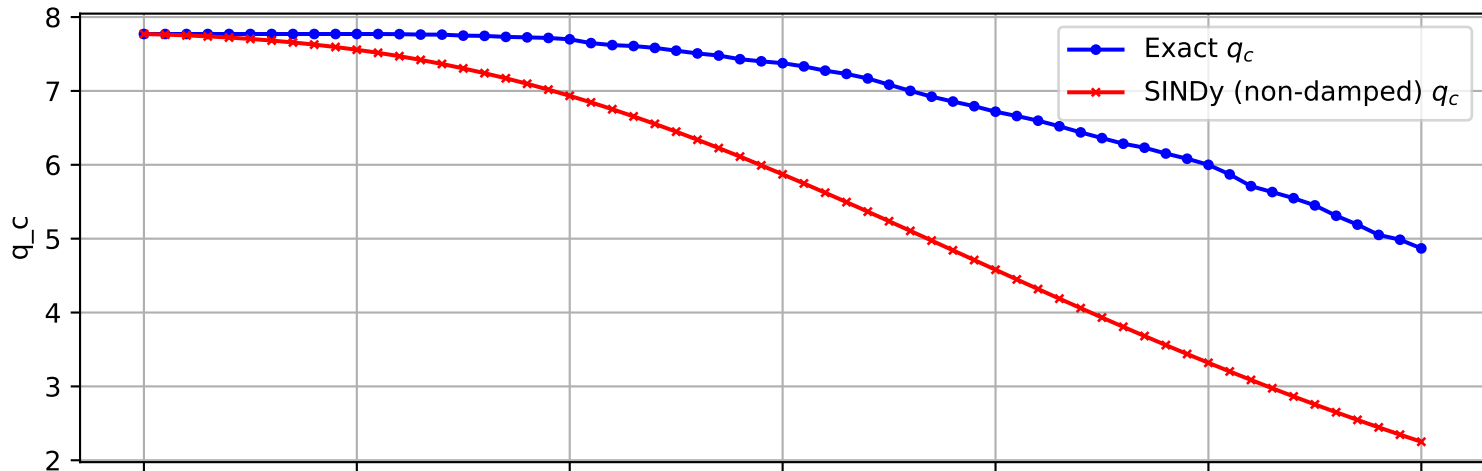
Trajectory 426 (non-damped)
