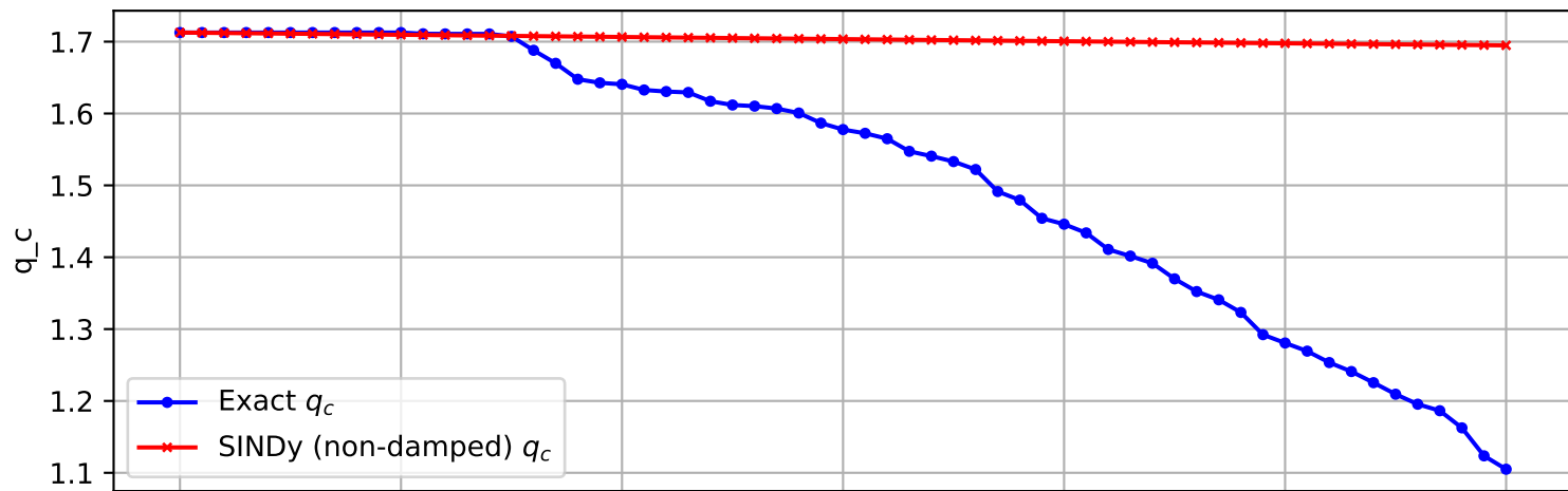
Trajectory 43 (non-damped)
