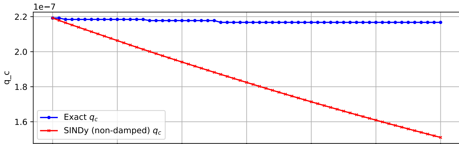
Trajectory 447 (non-damped)
