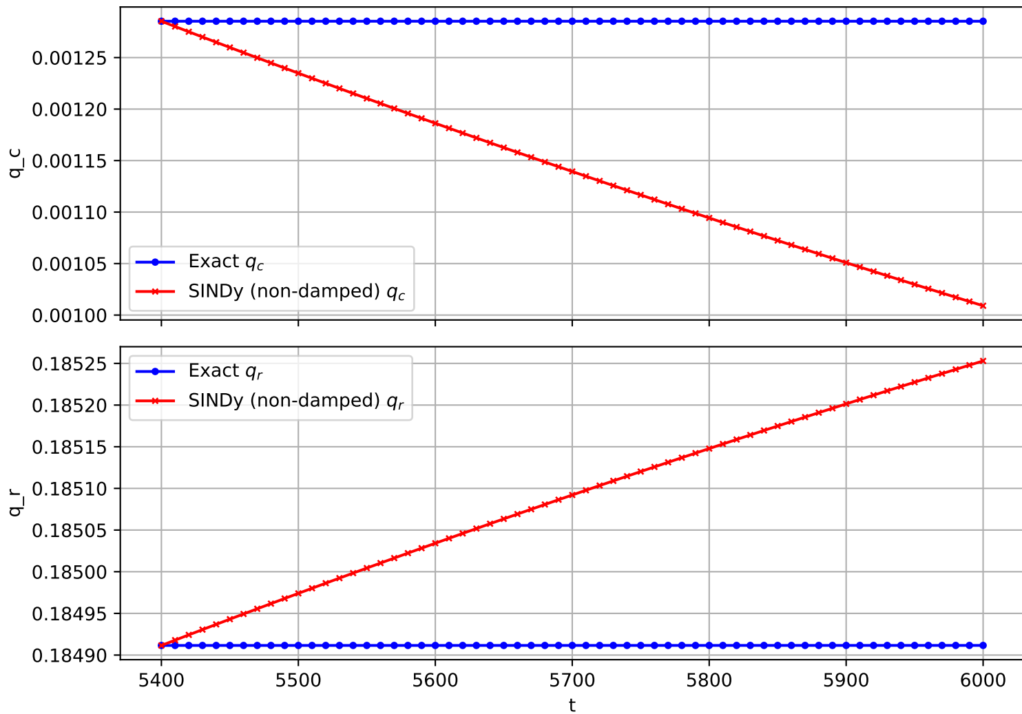
Trajectory 448 (non-damped)
