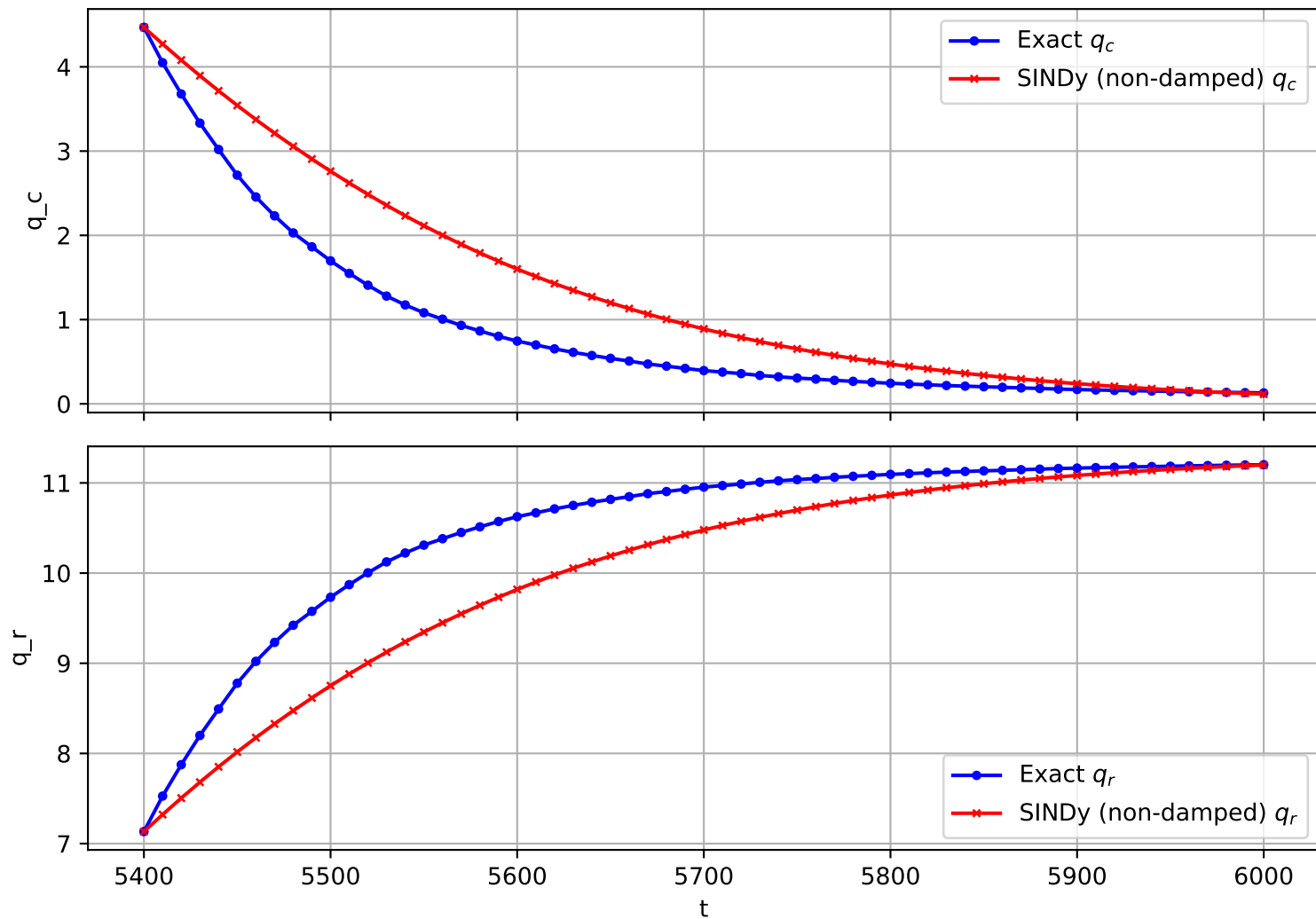
Trajectory 469 (non-damped)
