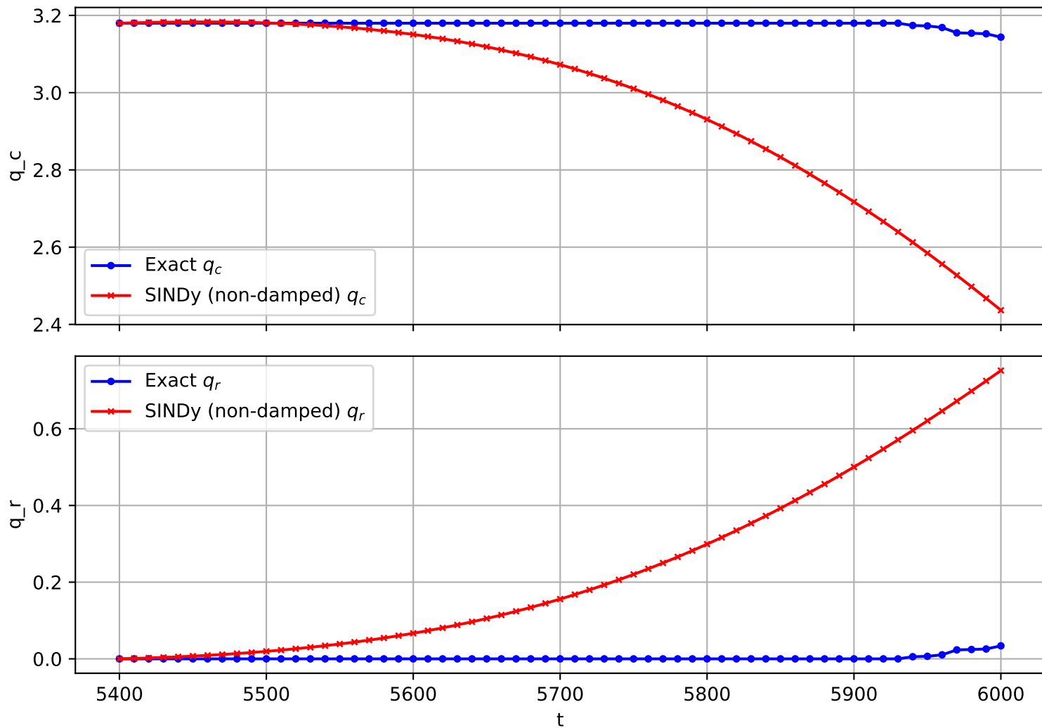
Trajectory 475 (non-damped)
