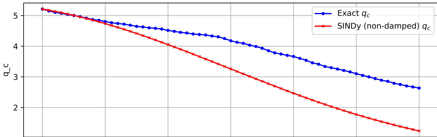
Trajectory 476 (non-damped)
