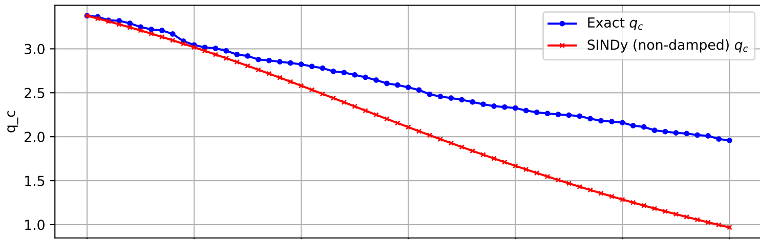
Trajectory 481 (non-damped)
