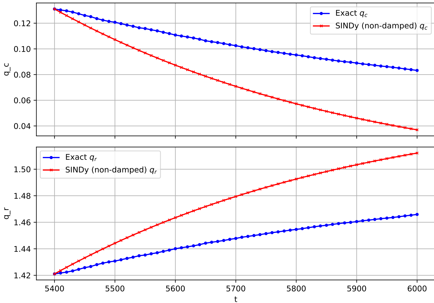
Trajectory 493 (non-damped)
