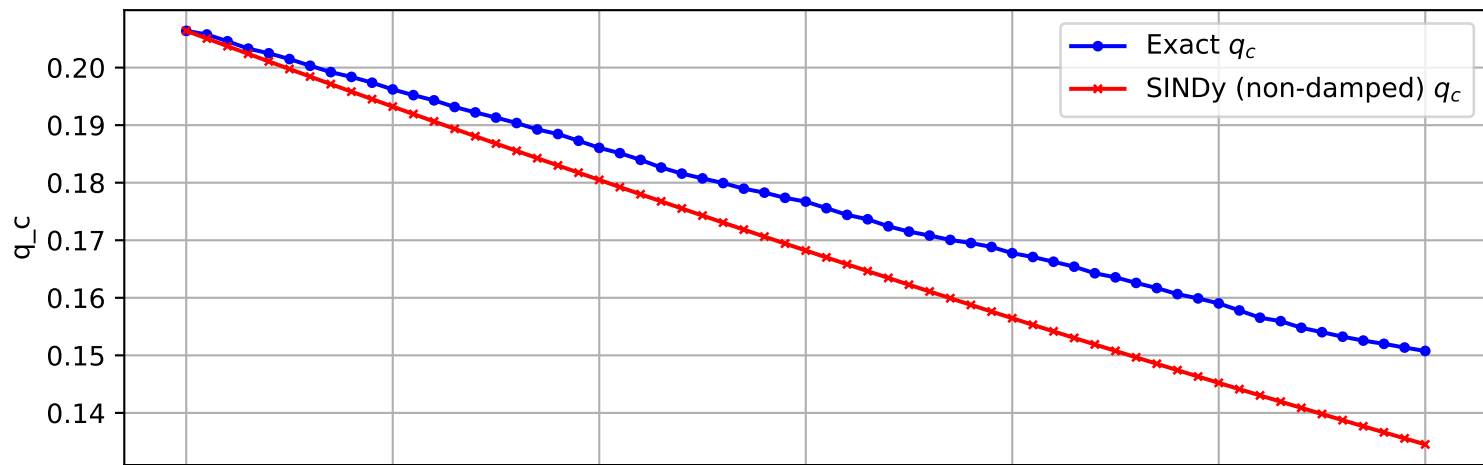
Trajectory 499 (non-damped)
