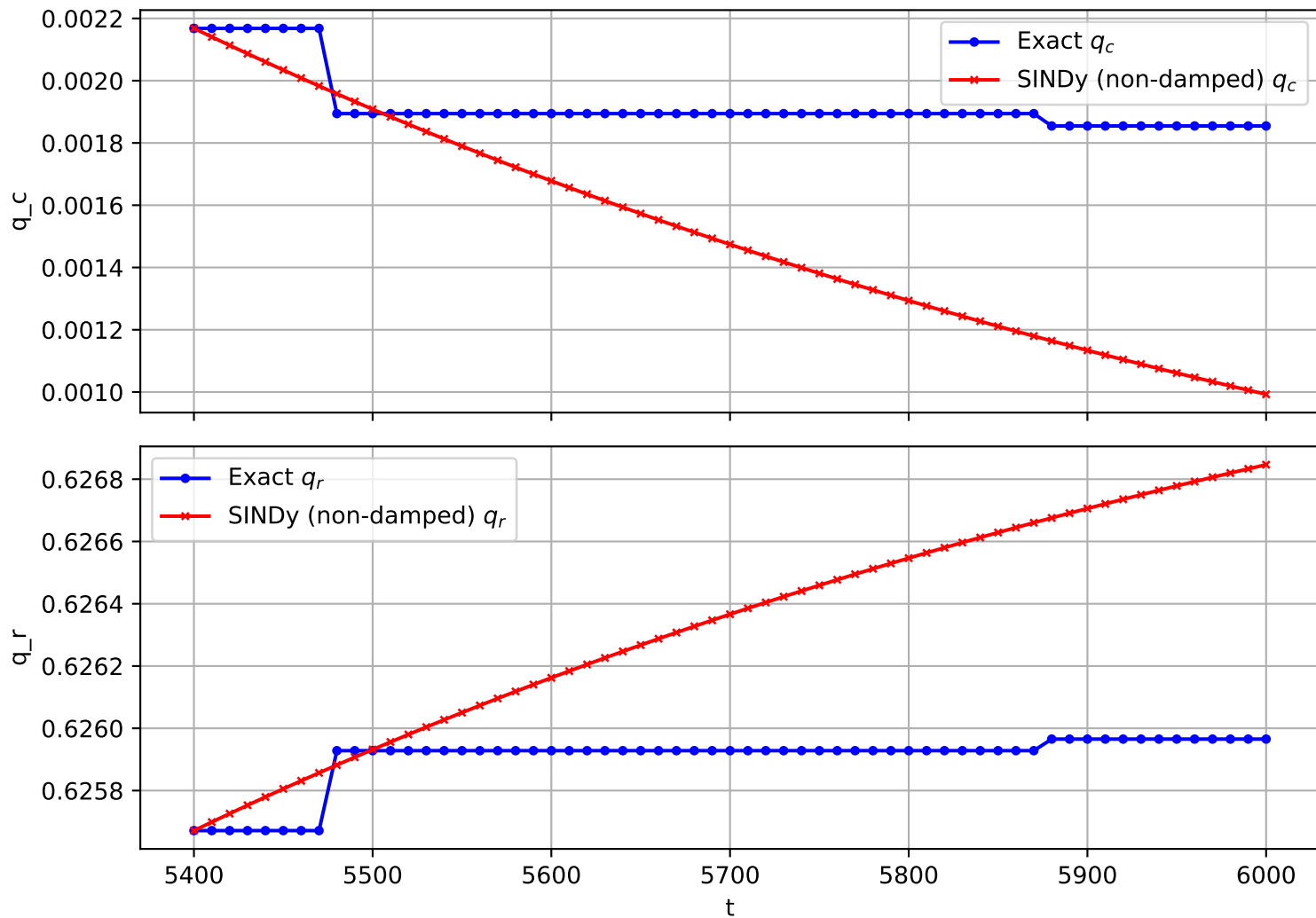
Trajectory 505 (non-damped)
